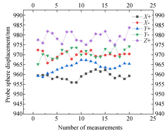
图 13 电容式三维纳米测量测头各方向测量重复性 Fig. 13 Repeatability testing of capacitive 3D nanoscale measurement probe in different directions
